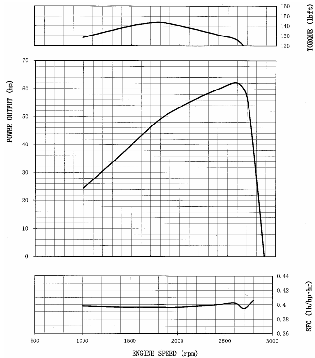
4JG1PK-01 Curve
