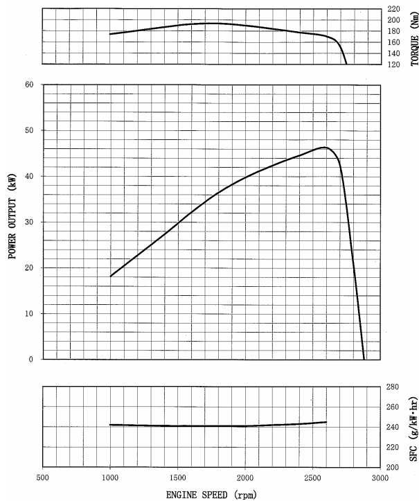
4JG1PK Curve
